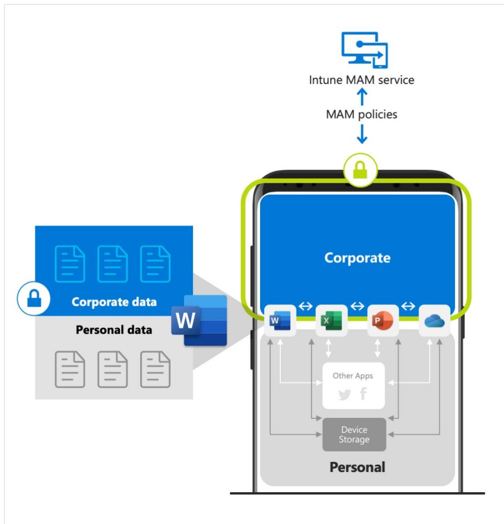
Figure 3: App protection policies provide app level protection
